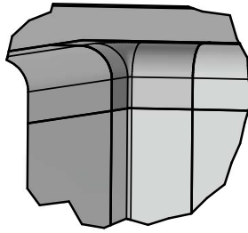
DETAIL A OUTSIDE 3-WAY 90° L RADIUS CORNER TRANSITION
