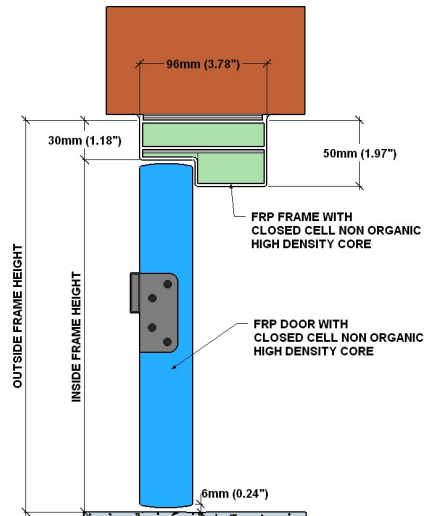
Side section detail, fixed to FRP frame
